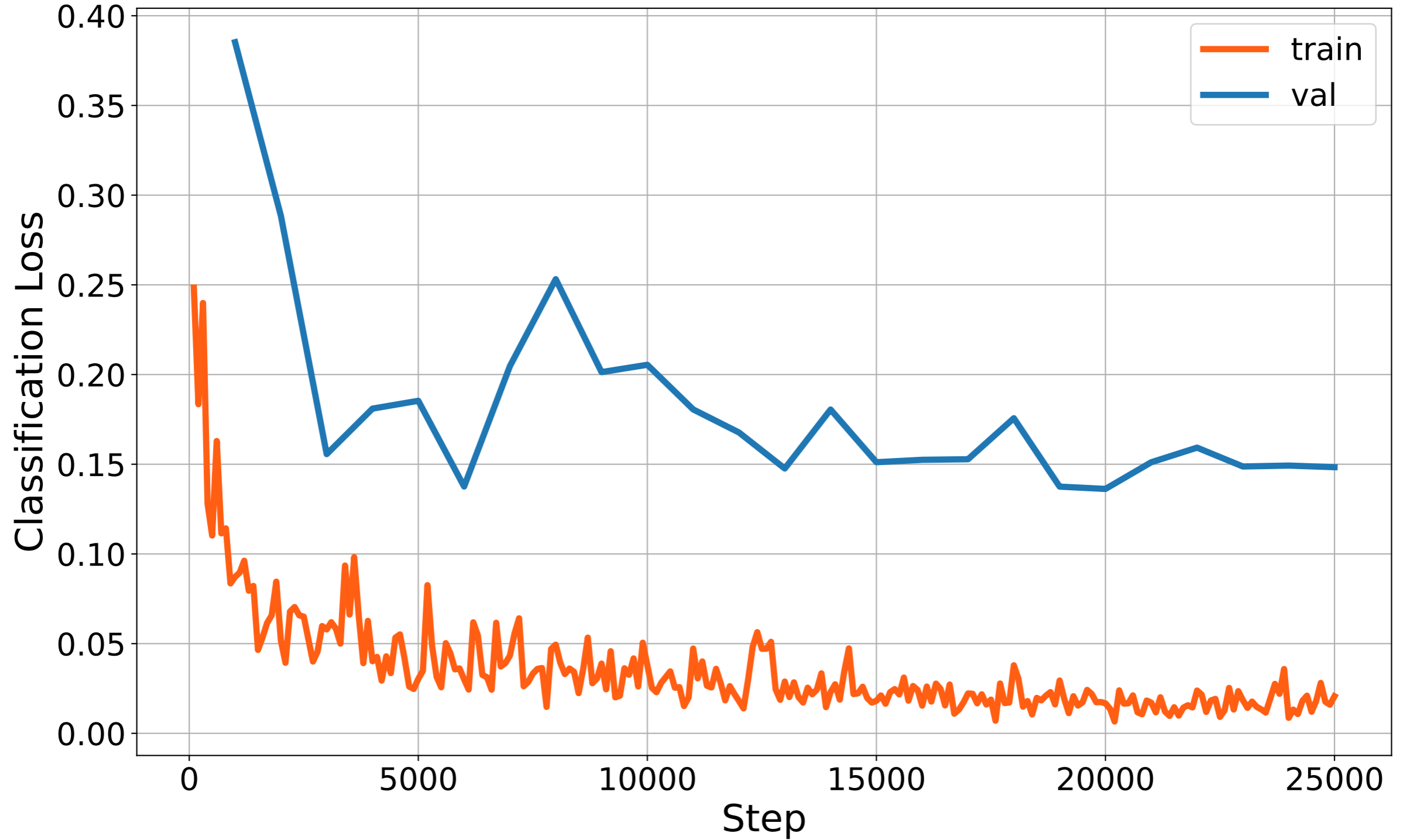
Classification Loss
